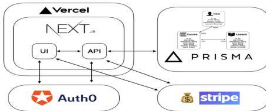
Figure 1: Architecture of Building a SaaS Application with Next.js, Prisma, Auth0, and Stripe.
