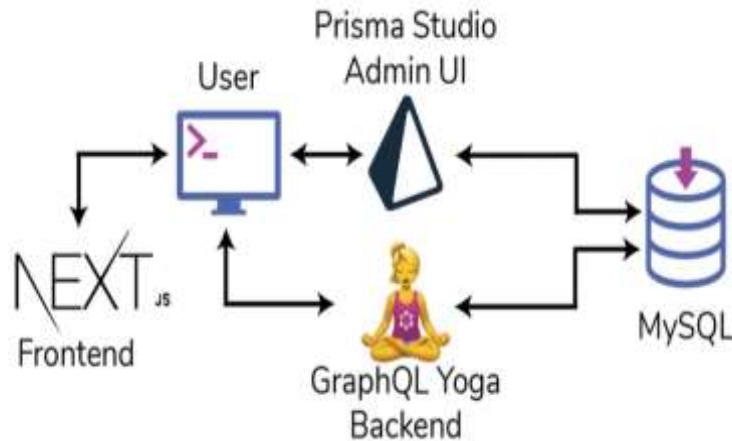
Figure 3: Architecture Overview of Web app with React, Next.JS, and Prisma 2.
