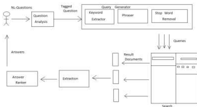
Fig. 1: System Architecture
