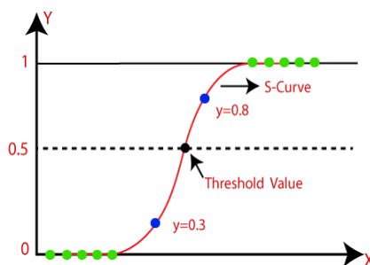
Fig.1 Logistic Regression
