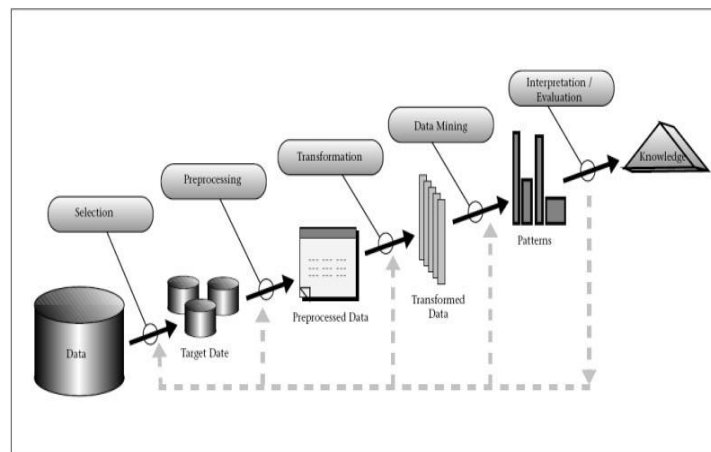
Figure1. Knowledge discovery Process
