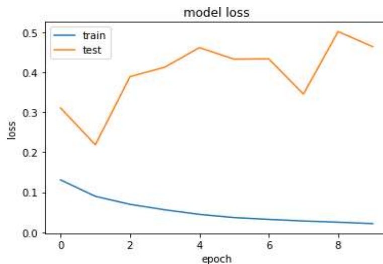
Fig.13: Loss plot for 2:1 Architecture without using Batch Normalization and Dropout
