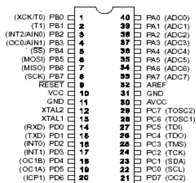
Fig 4 ATMEGA 16
