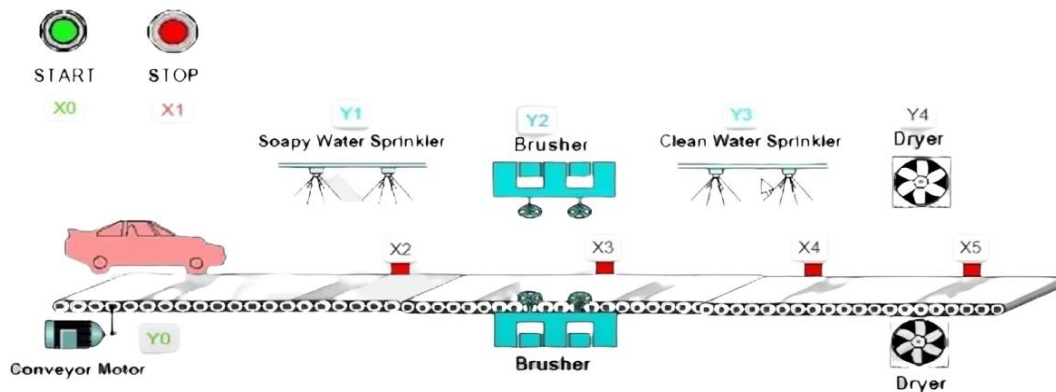
Figure 1: Working of car wash system
