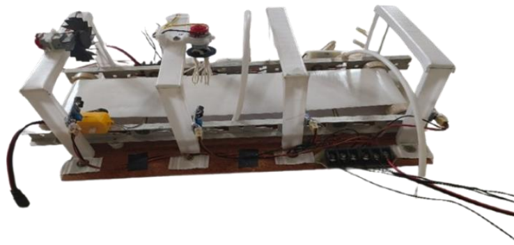
Figure 3: Working model of car wash system
