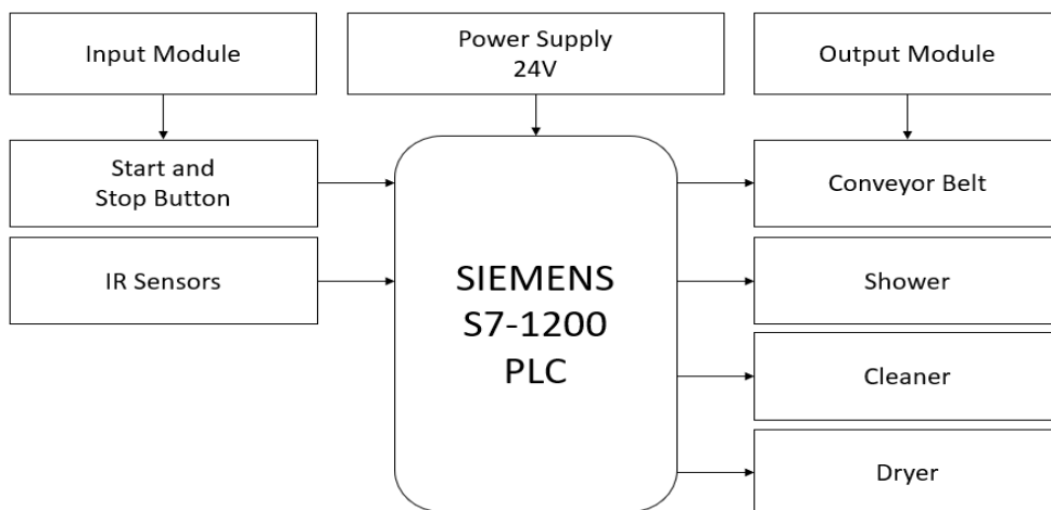
Figure 2: Block diagram of car wash system
