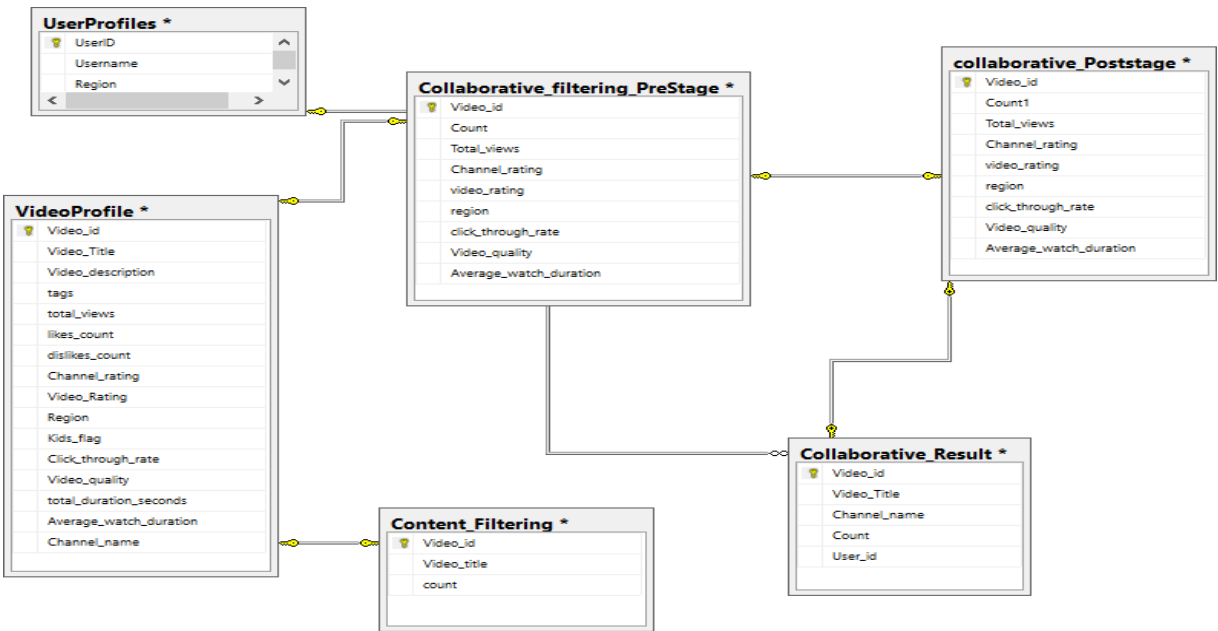
Figure 2 : Database Design
