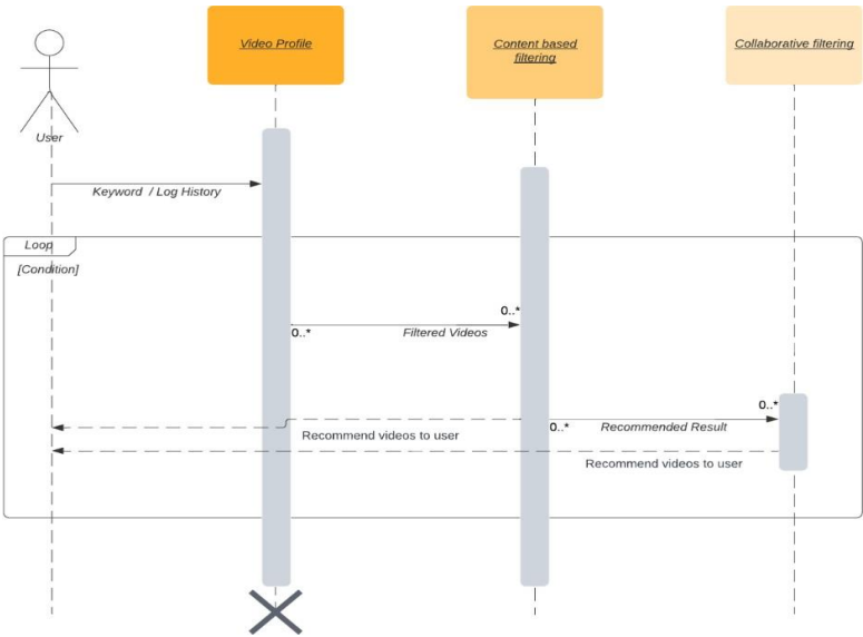
Figure 1. Sequence diagram
