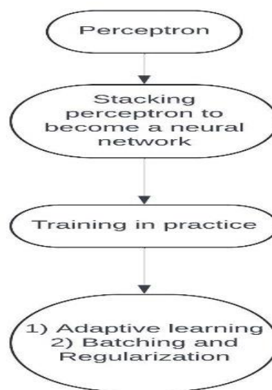
Figure 2. Perceptron aggregation
